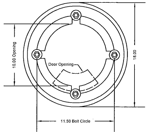
C Anchore Bolt Detail Not to Scale
