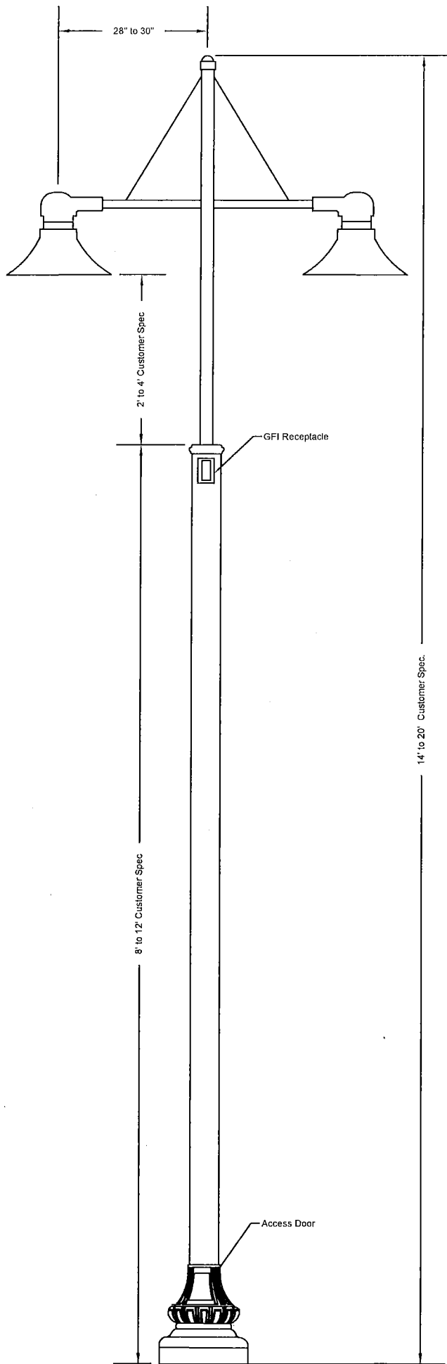
A Light Pole Detail Not to Scale
