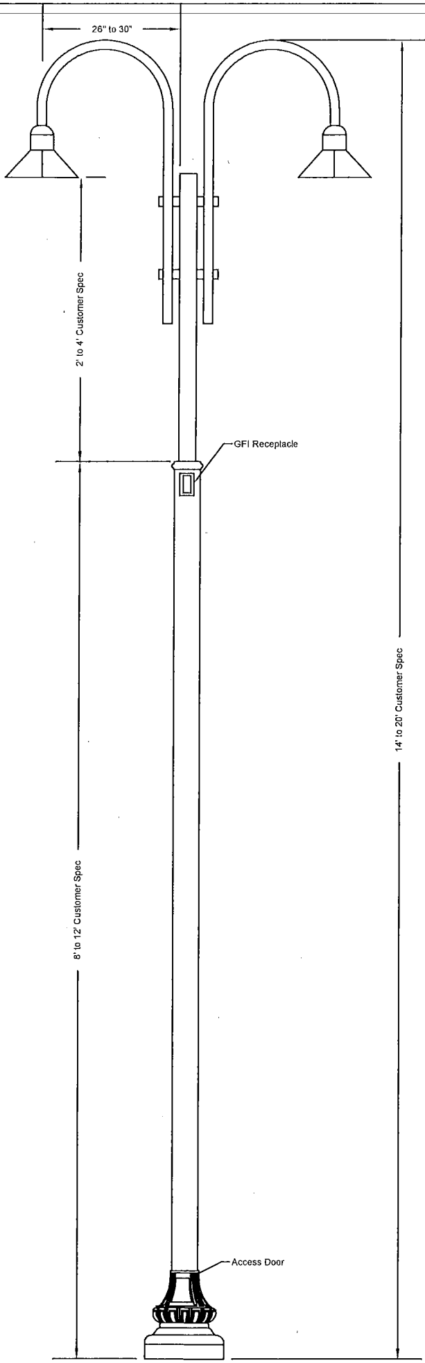
A Light Pole Detail Not to Scale
